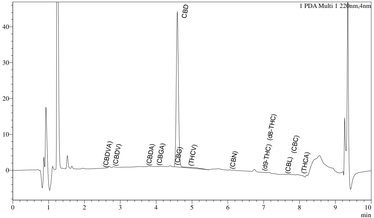
Chromatogram
